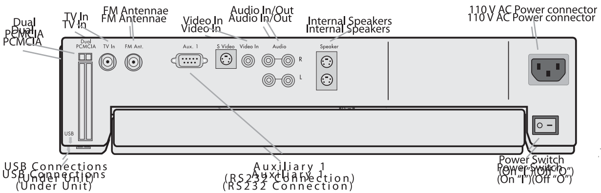
FIGURE 5. Rear Panel of the iCEBOX FlipScreen
